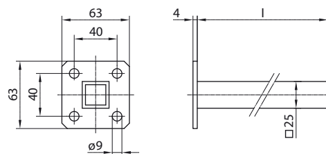
Towing arm
