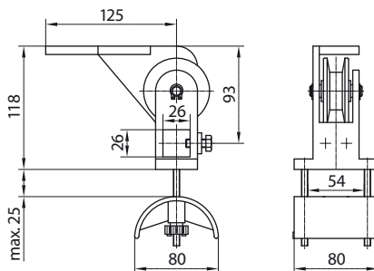
Towing trolley
