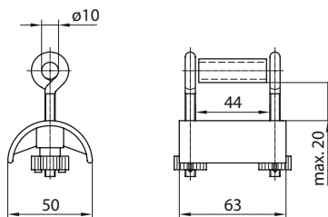
Cable support
