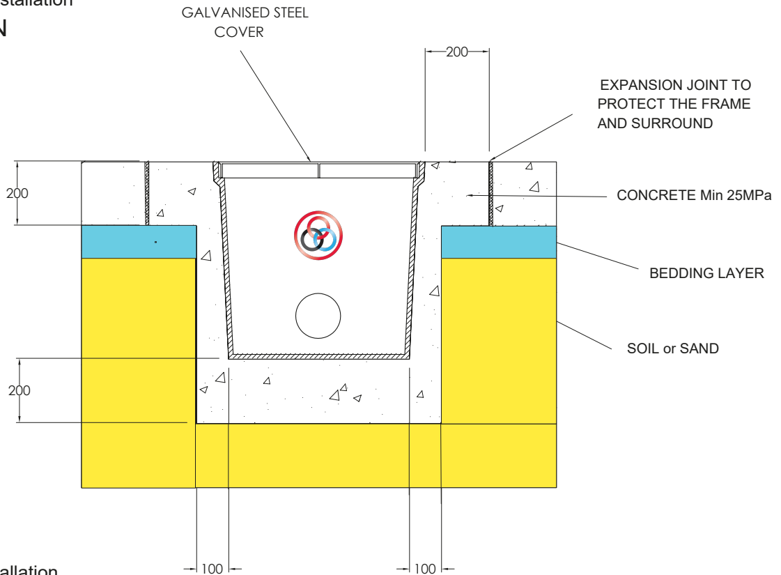
Class D Installation 210kN
